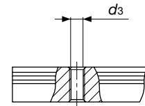
Tapped rail specification LWL...N
