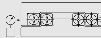
Fig. 3 Example of preload adjustment
