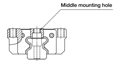
Fig.1 Middle mounting hole of slide unit
